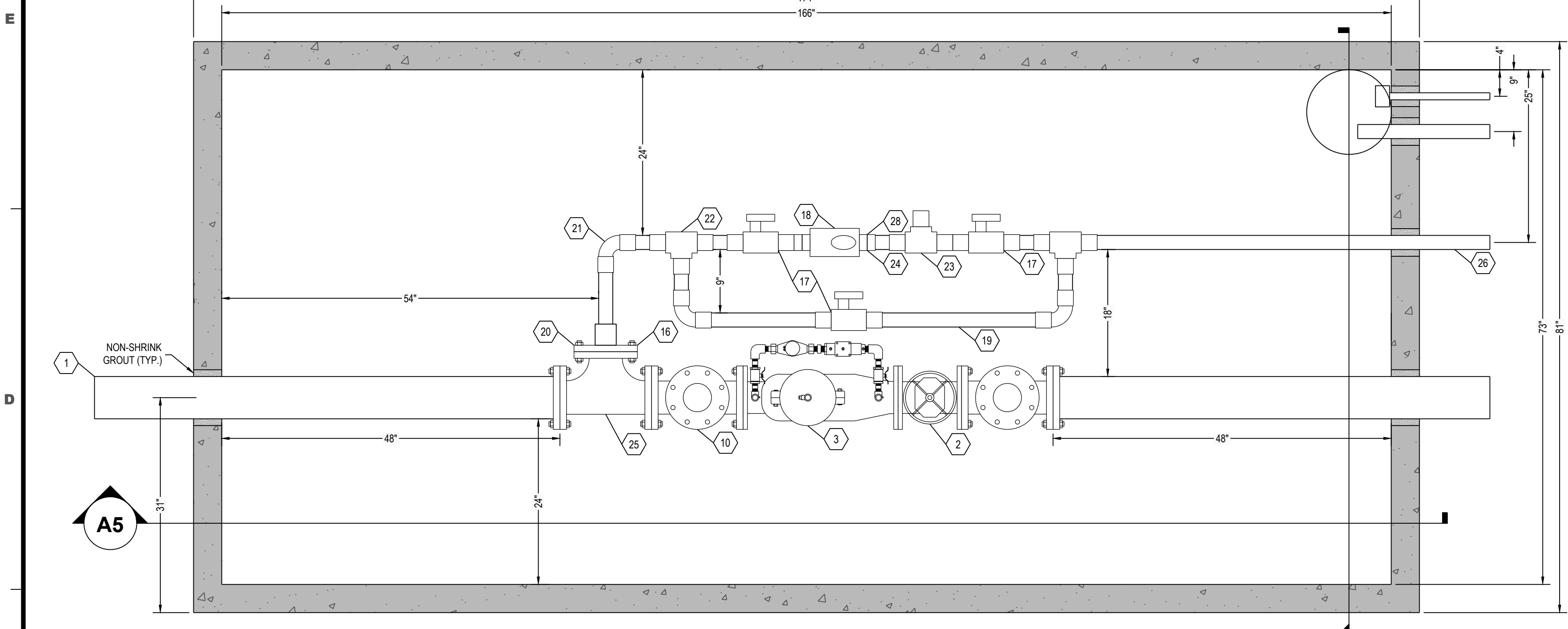
C6 WATER METER VAULT TOP VIEW 1" = 1"
