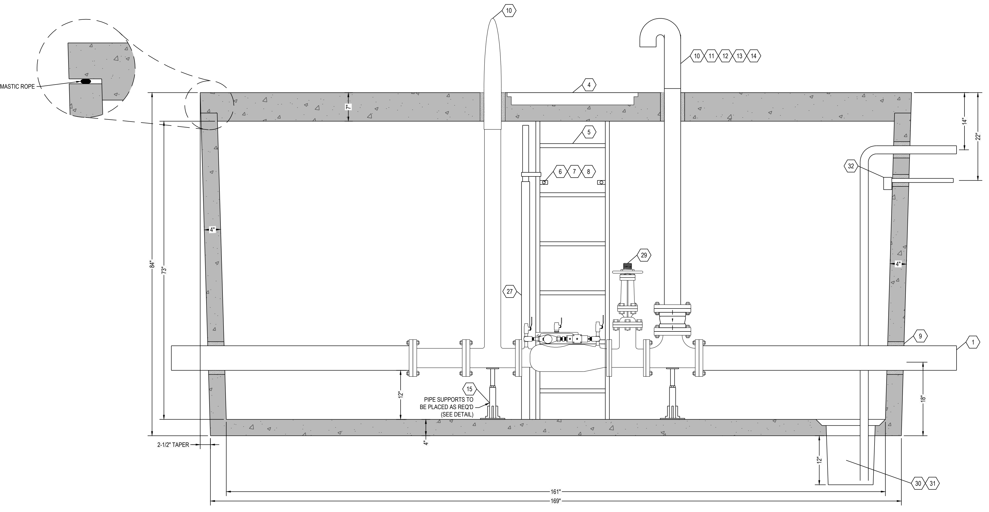
A5 WATER METER VAULT SECTION VIEW 1" = 1"
