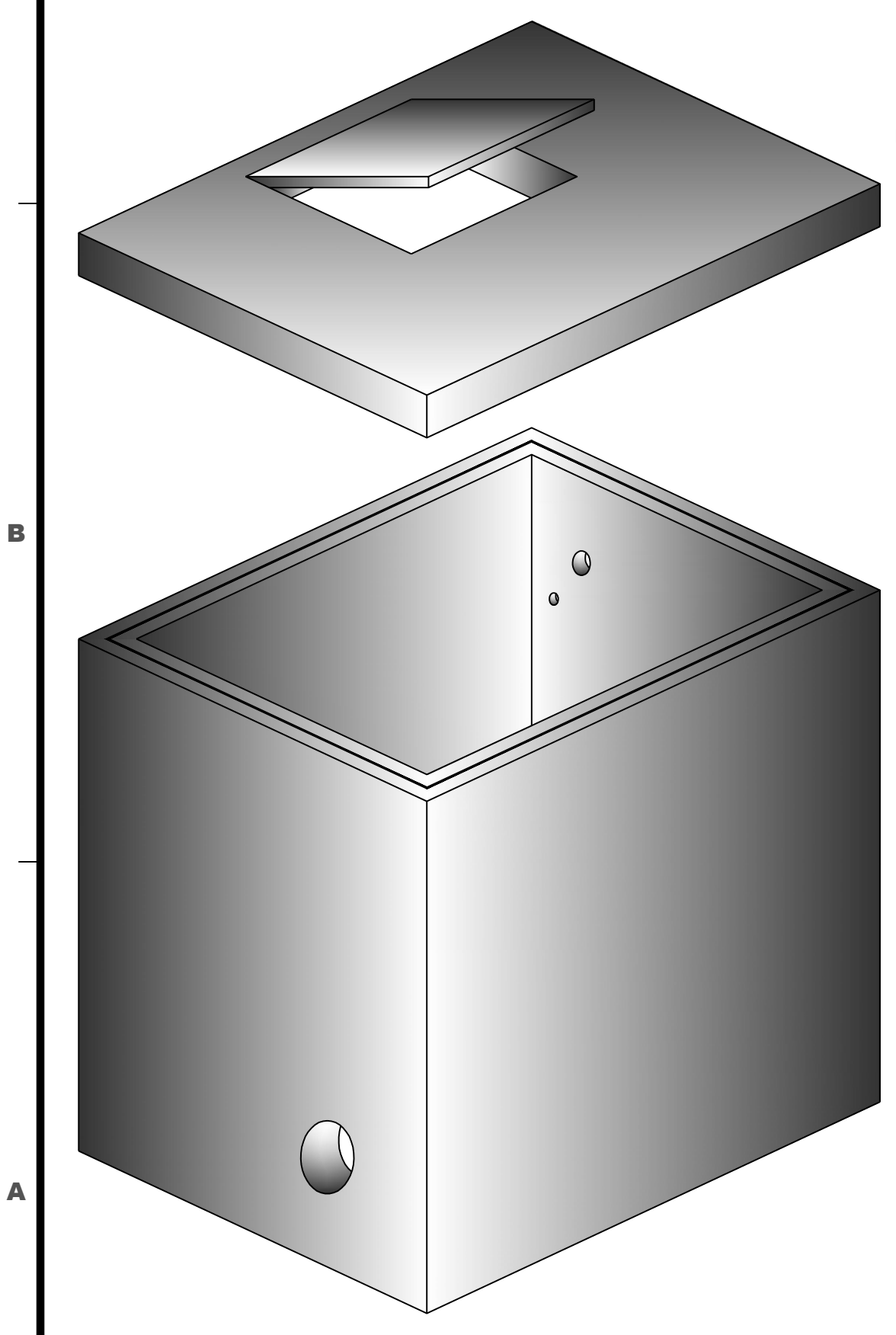
A6 THREE DIMENSIONAL ISOMETRIC VIEW NTS
