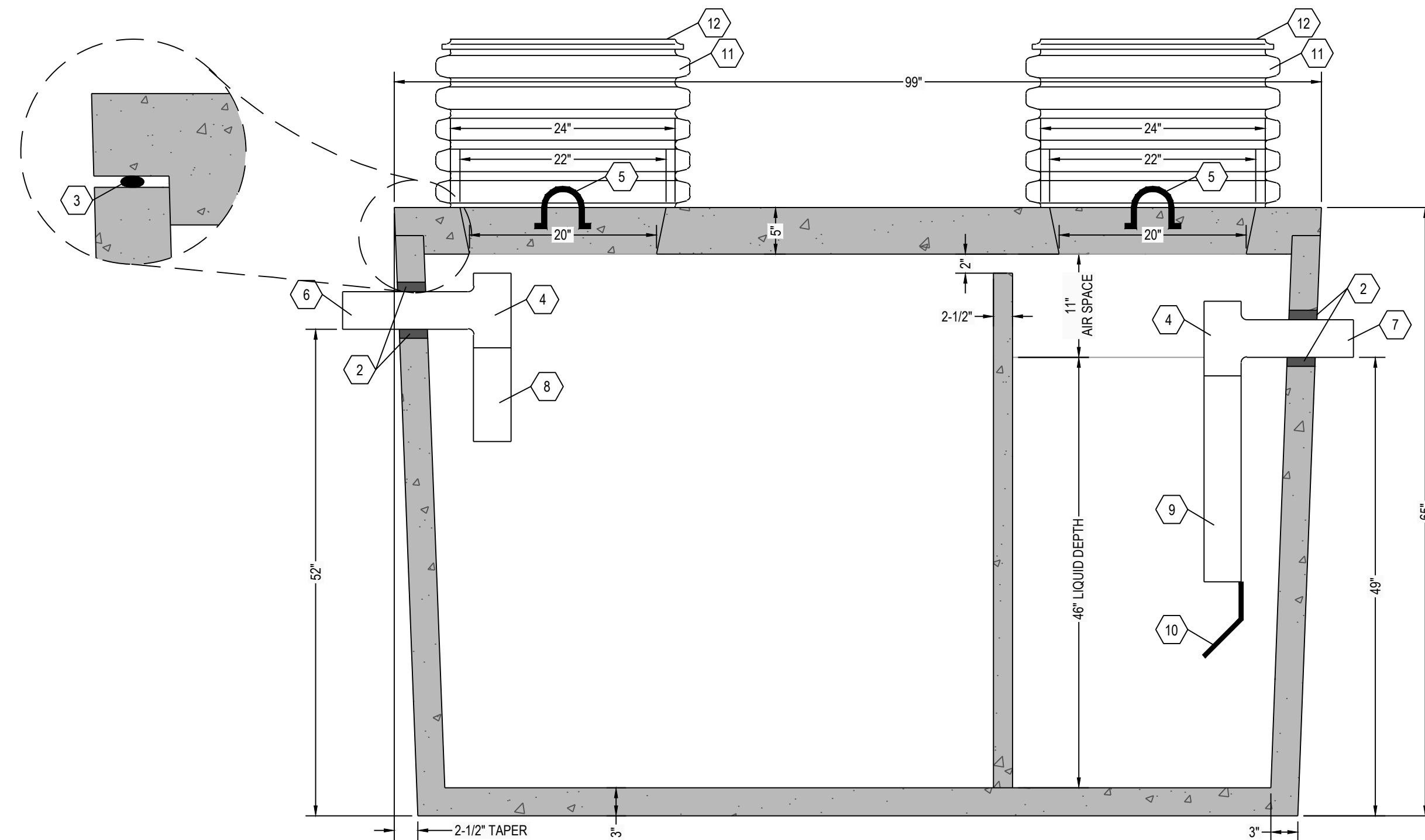
A5 SEPTIC TANK SECTION VIEW 1" = 1"
