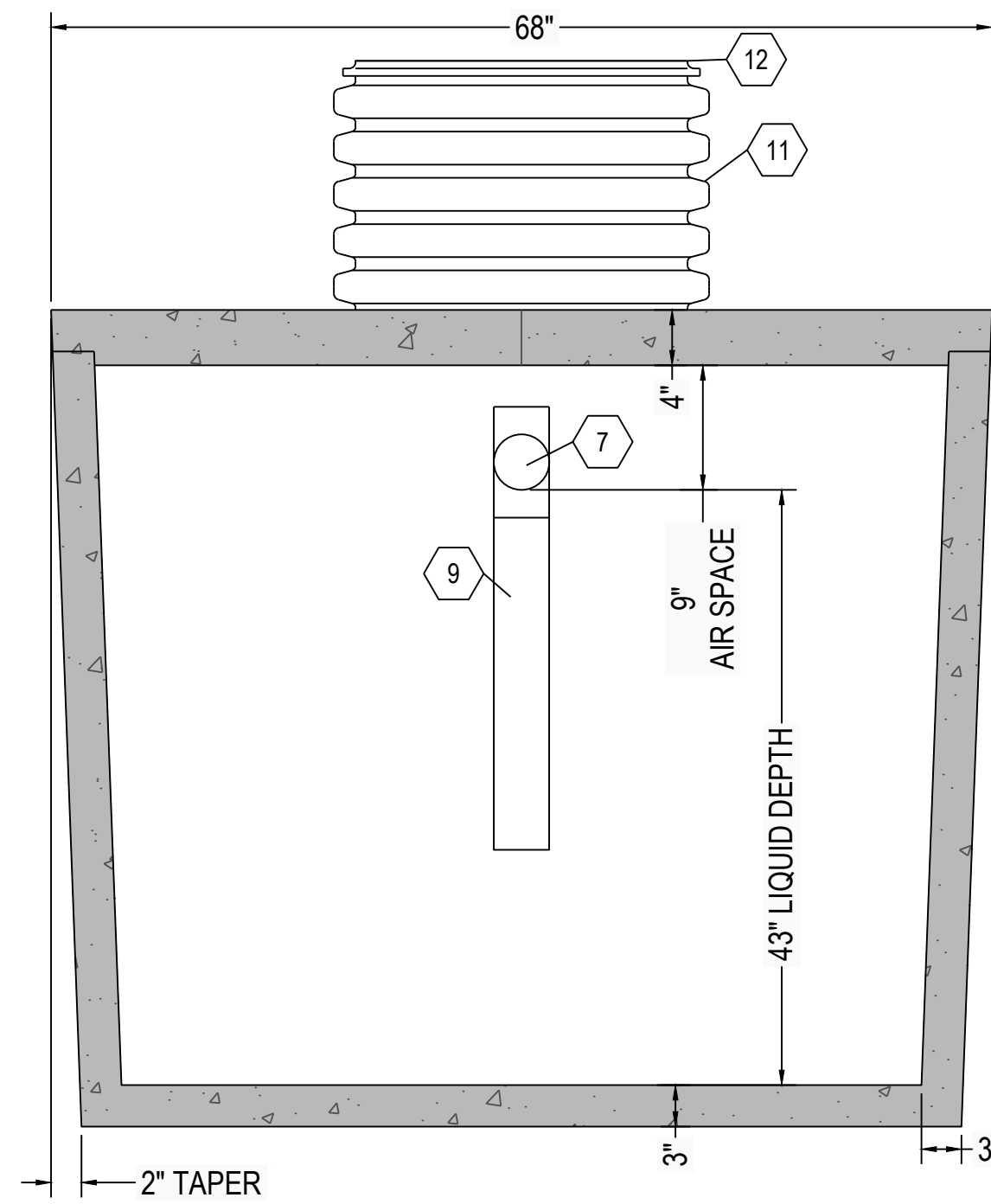
C4 SEPTIC TANK SECTION VIEW 1" = 1"
