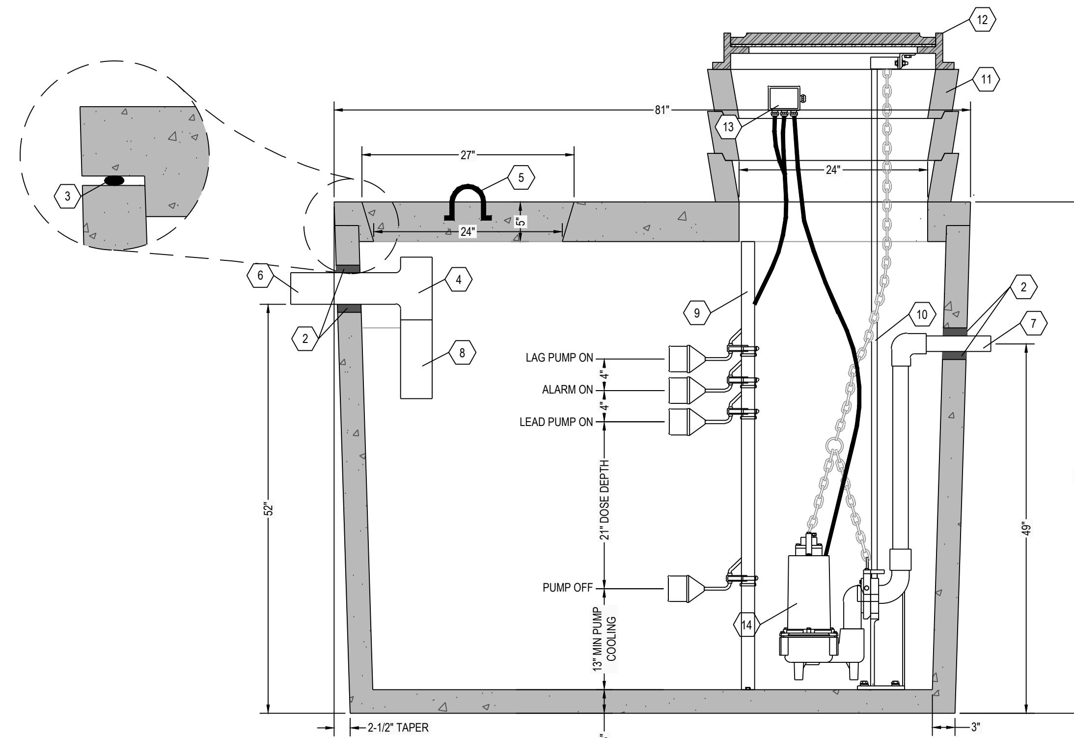
A5 SEPTIC TANK SECTION VIEW 1" = 1"
