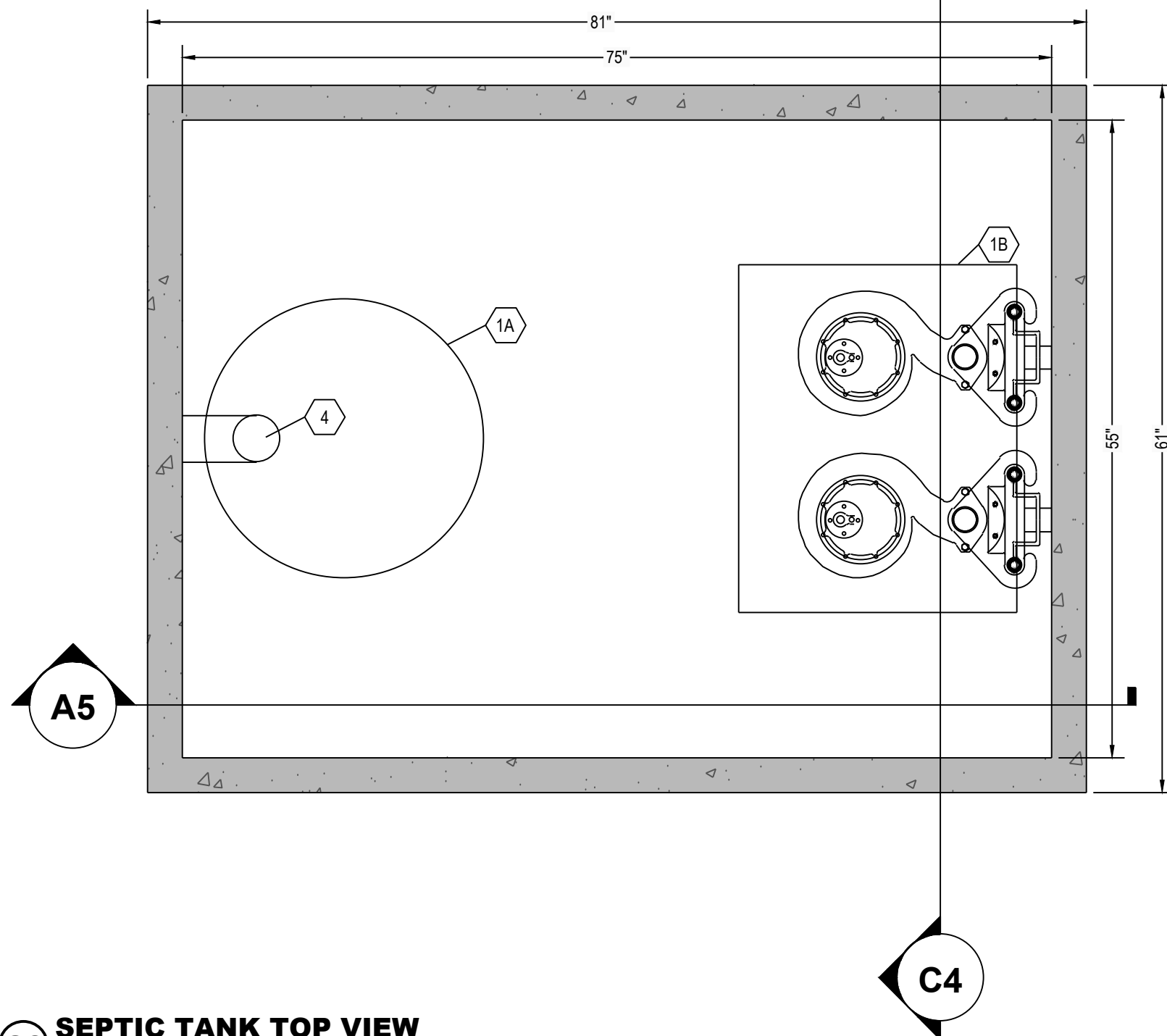
C6 SEPTIC TANK TOP VIEW 1" = 1"
