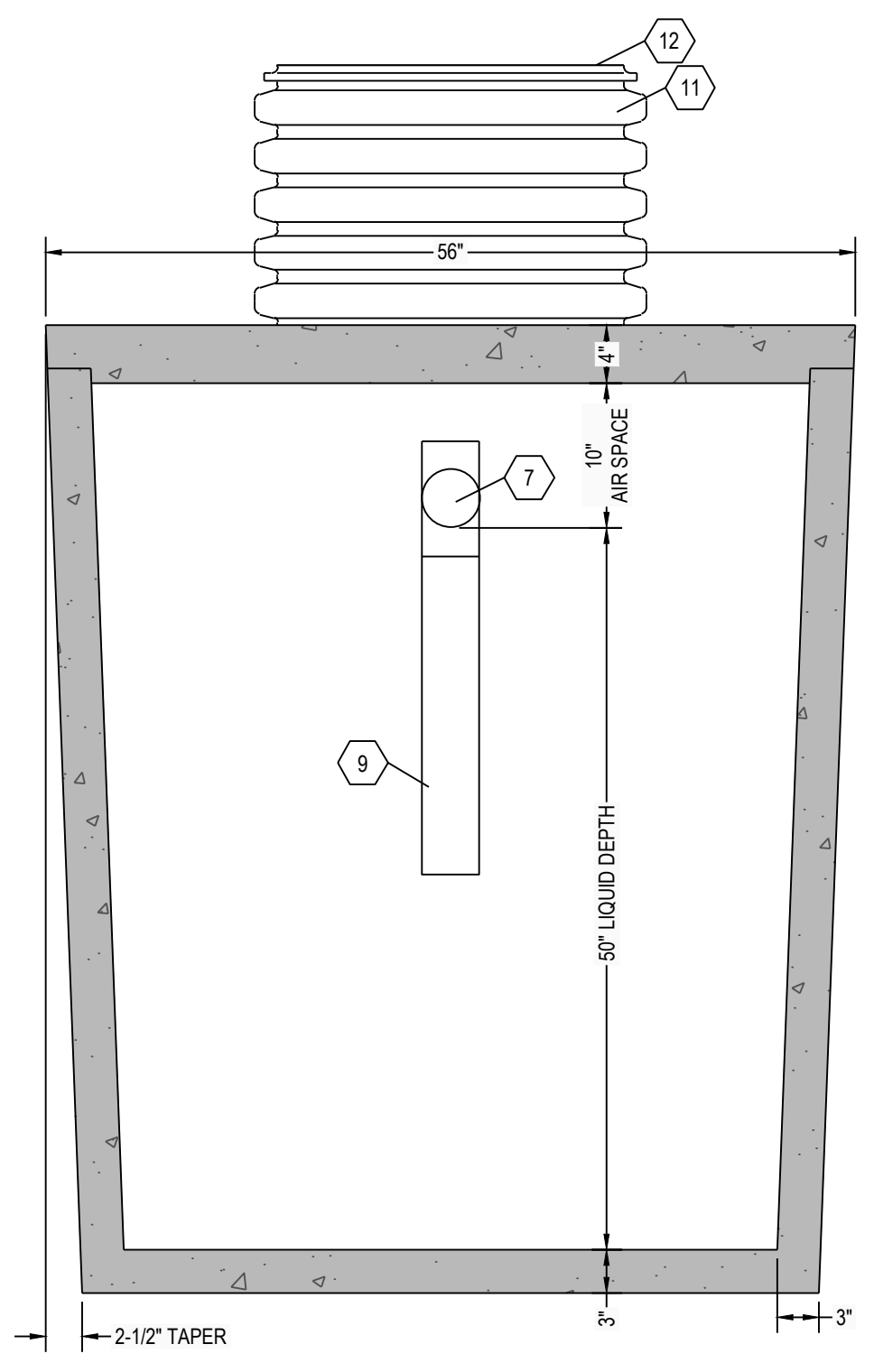
C4 SEPTIC TANK SECTION VIEW 1" = 1"
