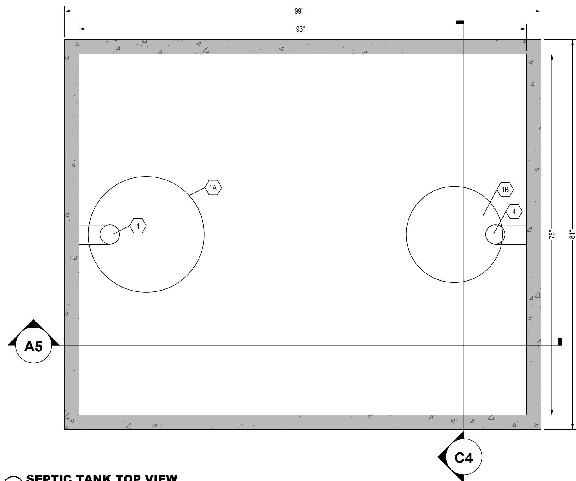
C6 SEPTIC TANK TOP VIEW 1" = 1"
