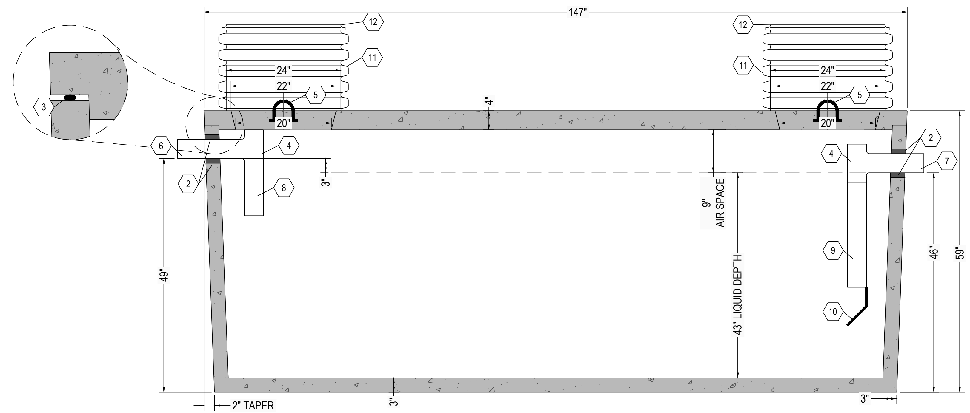
A5 SEPTIC TANK SECTION VIEW 1" = 1"
