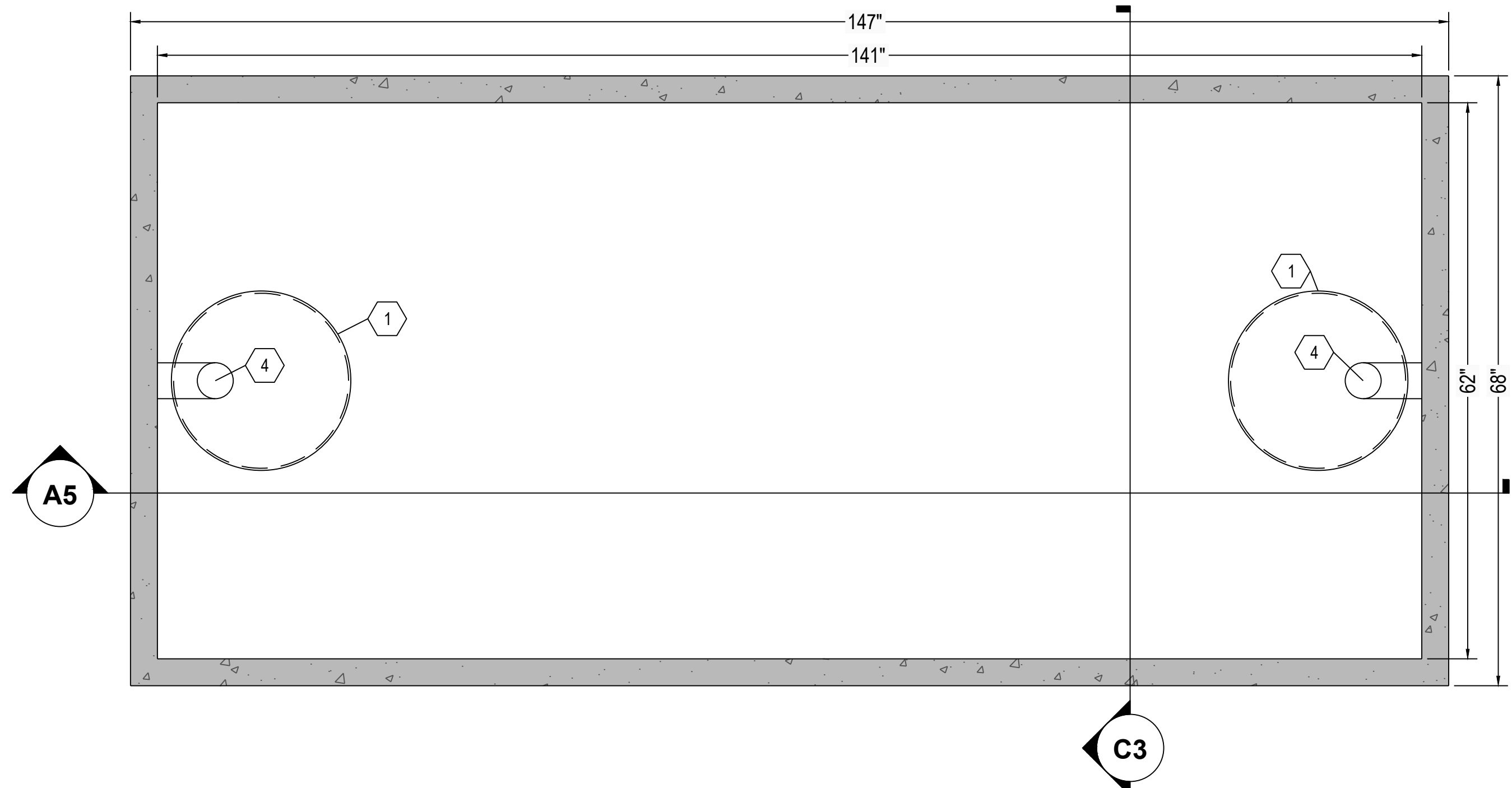
C6 SEPTIC TANK TOP VIEW 1" = 1"
