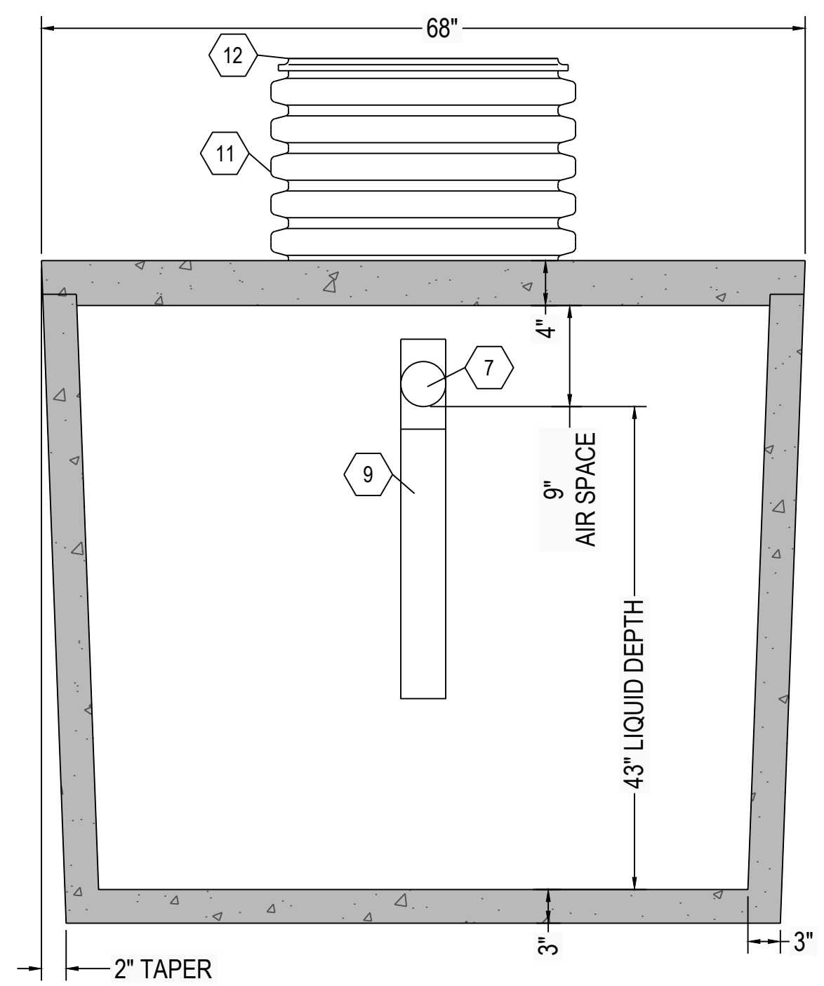
C4 SEPTIC TANK SECTION VIEW 1" = 1"
