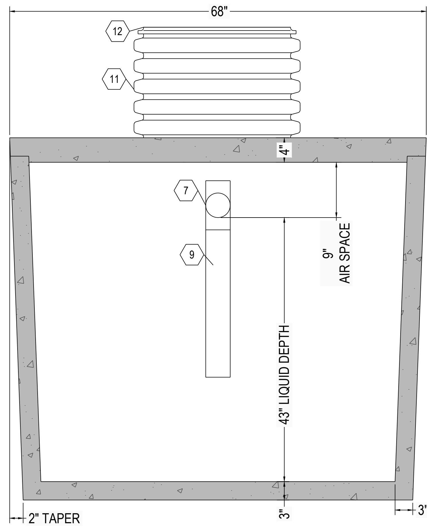
C4 SEPTIC TANK SECTION VIEW NTS
