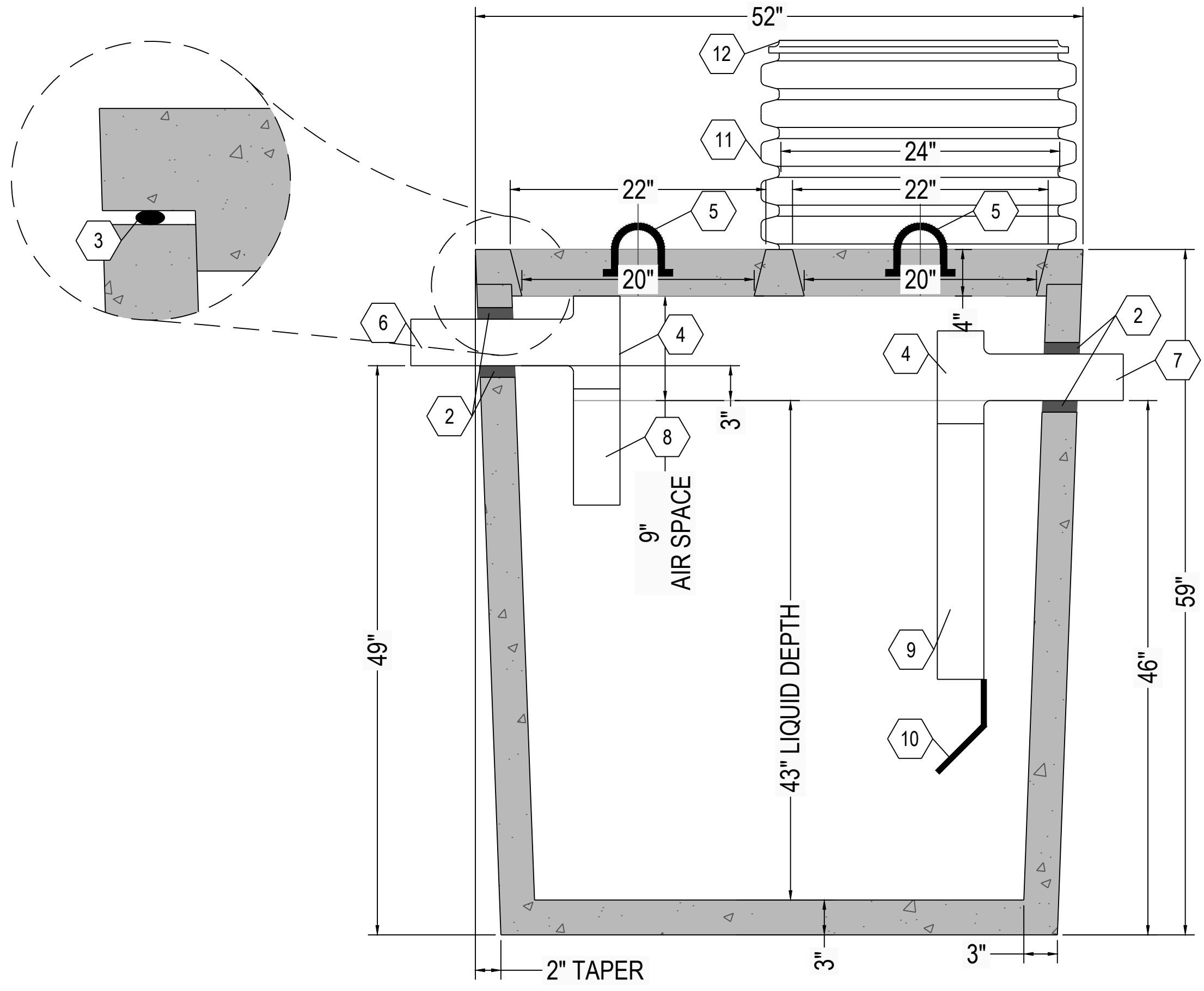
A5 SEPTIC TANK SECTION VIEW NTS
