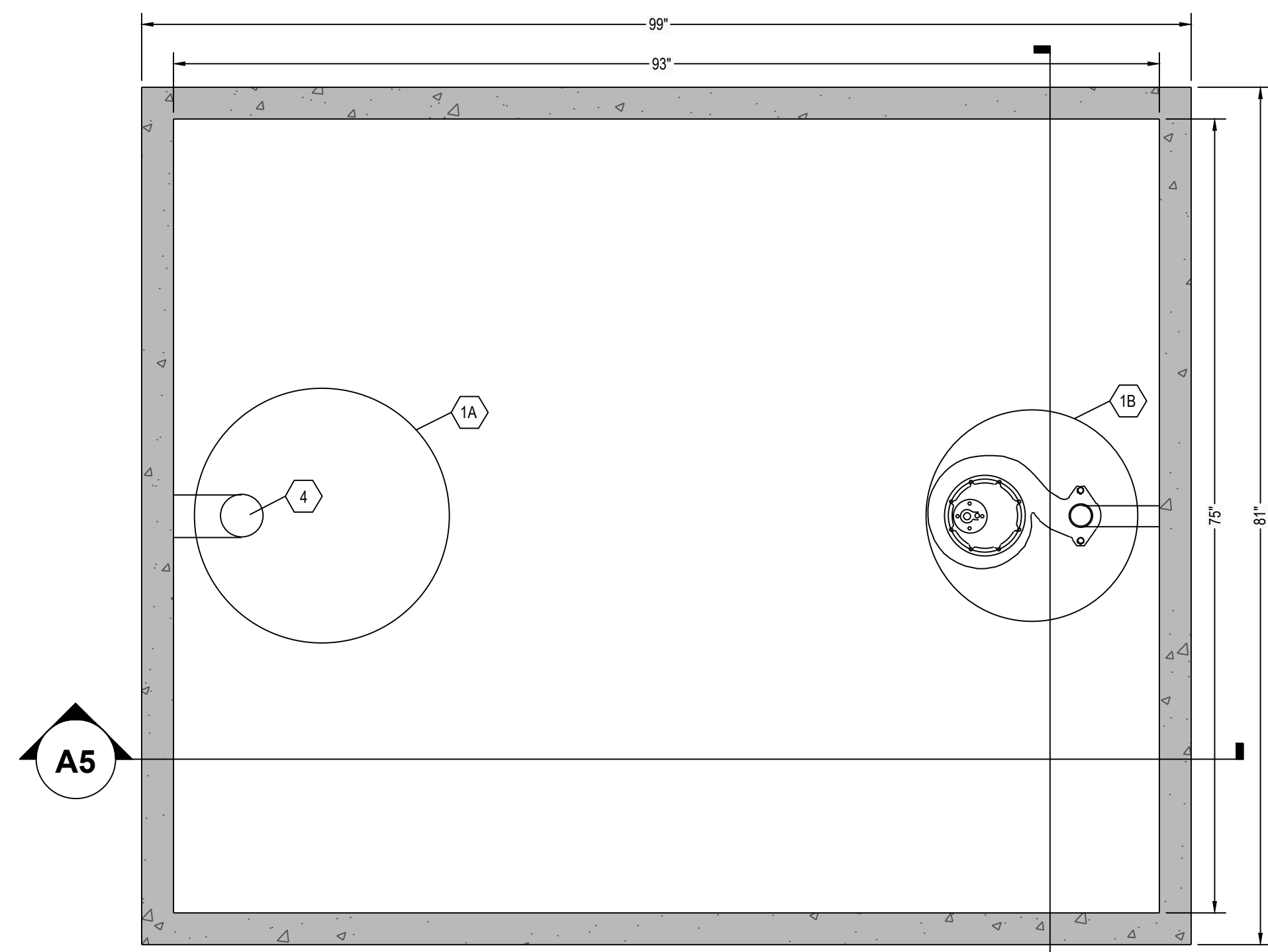
C6 SEPTIC TANK TOP VIEW 1" = 1"
